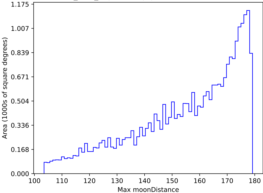
baseline_v2.1_10yrs All sky g band: Max moonDistance
