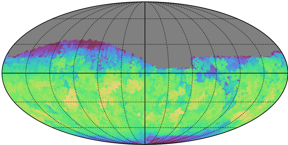
baseline_v2.1_10yrs Yr 1 z band: Max fiveSigmaDepth
