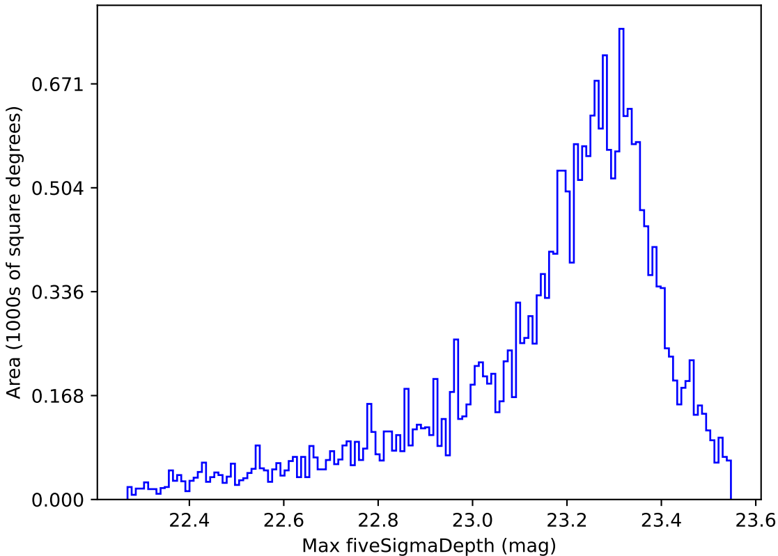
baseline_v2.1_10yrs Yr 1 z band: Max fiveSigmaDepth
