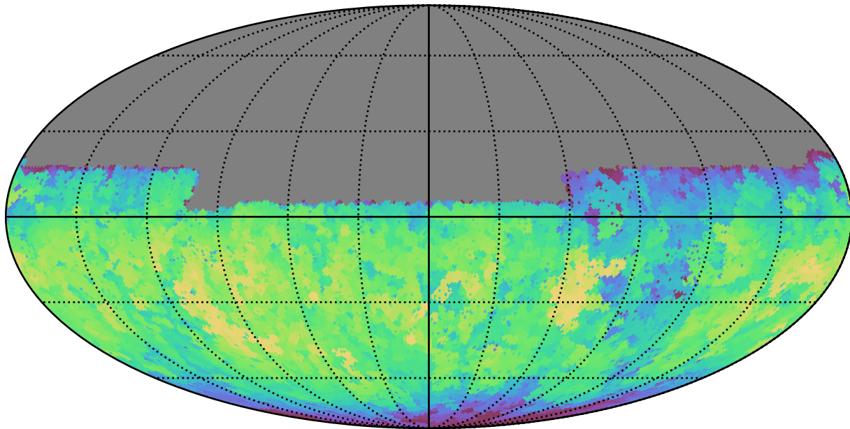
baseline_v2.1_10yrs Yr 1 y band: Max fiveSigmaDepth
