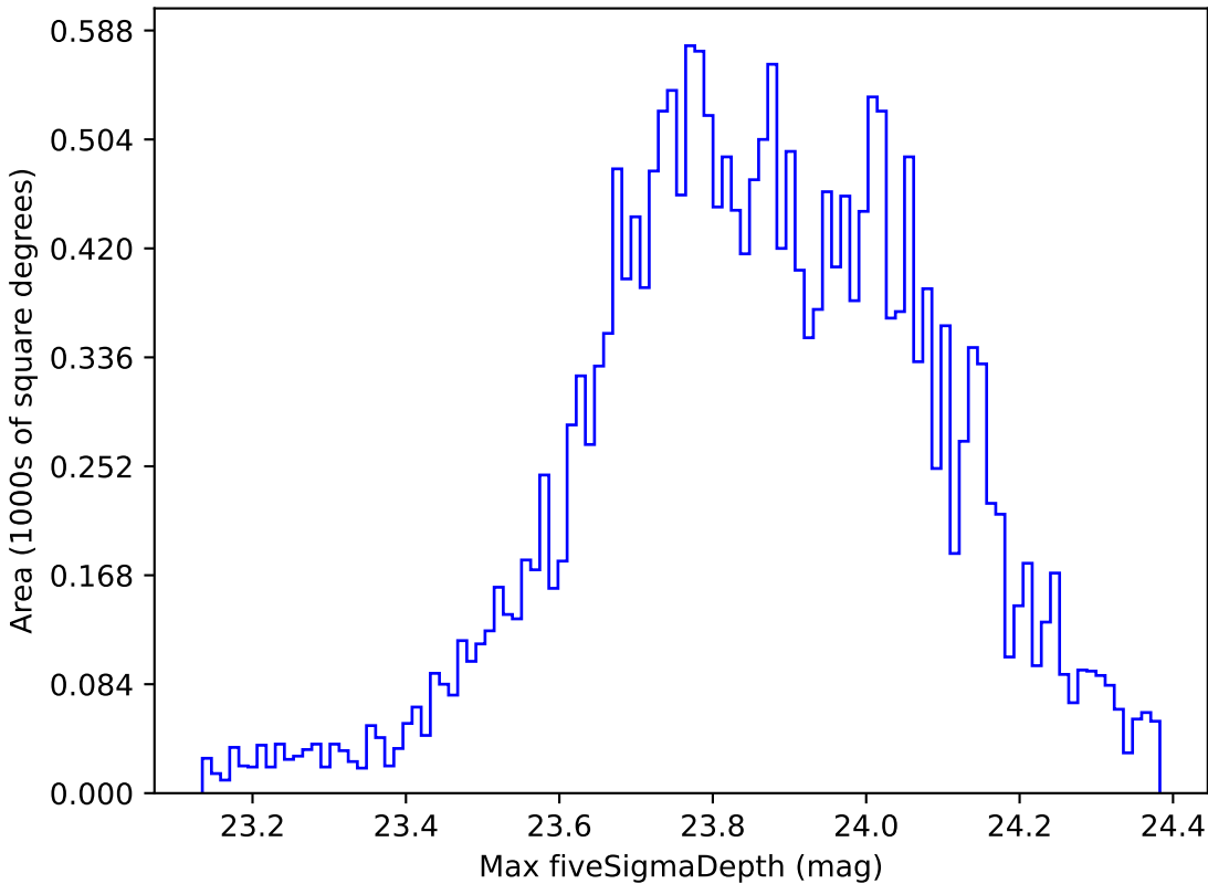
baseline_v2.1_10yrs Yr 1 u band: Max fiveSigmaDepth
