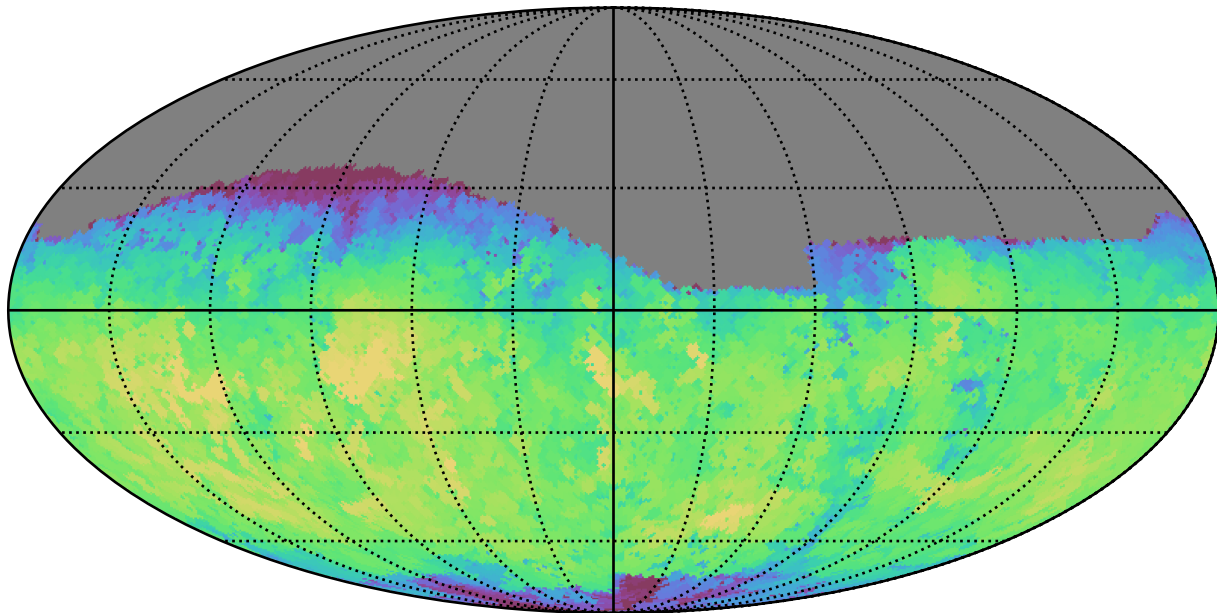
baseline_v2.1_10yrs Yr 1 r band: Max fiveSigmaDepth
