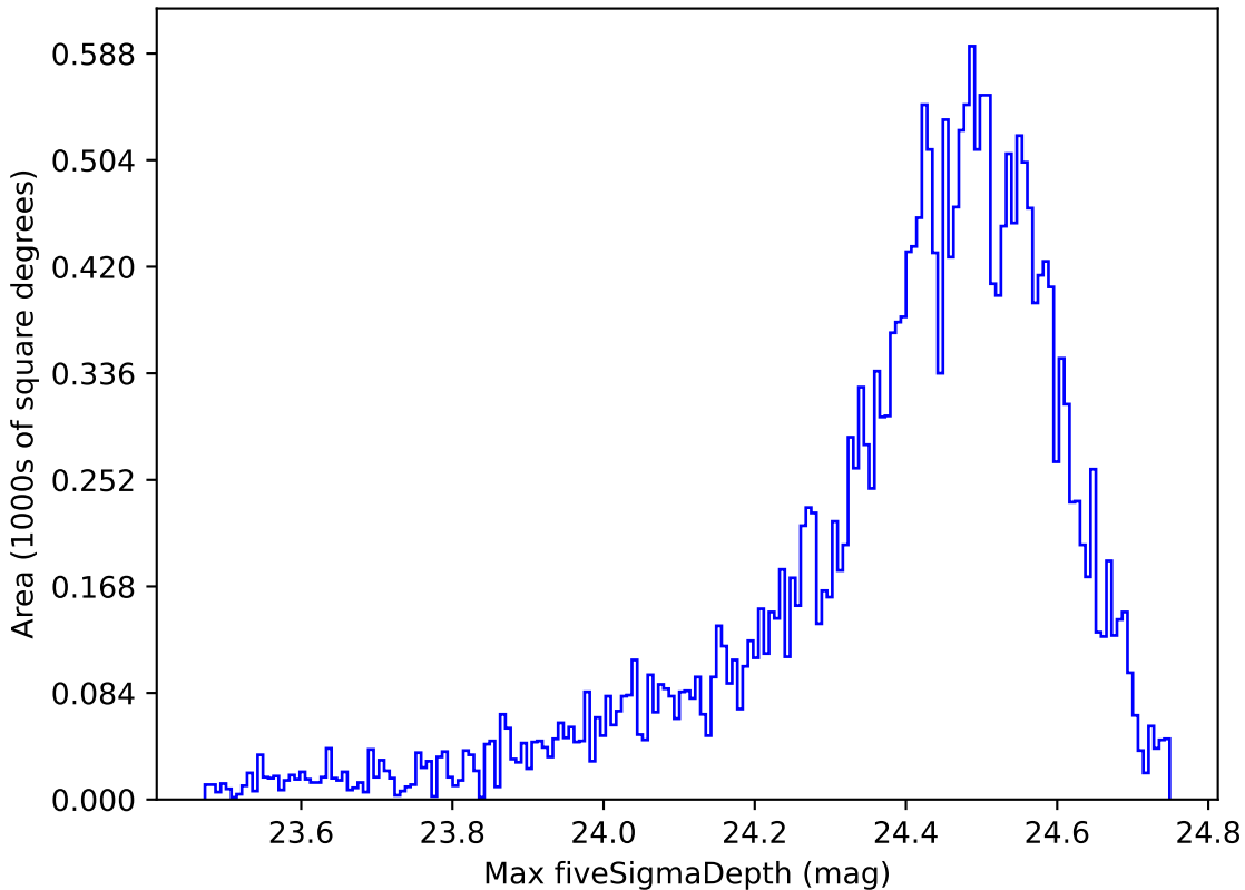
baseline_v2.1_10yrs Yr 1 r band: Max fiveSigmaDepth
