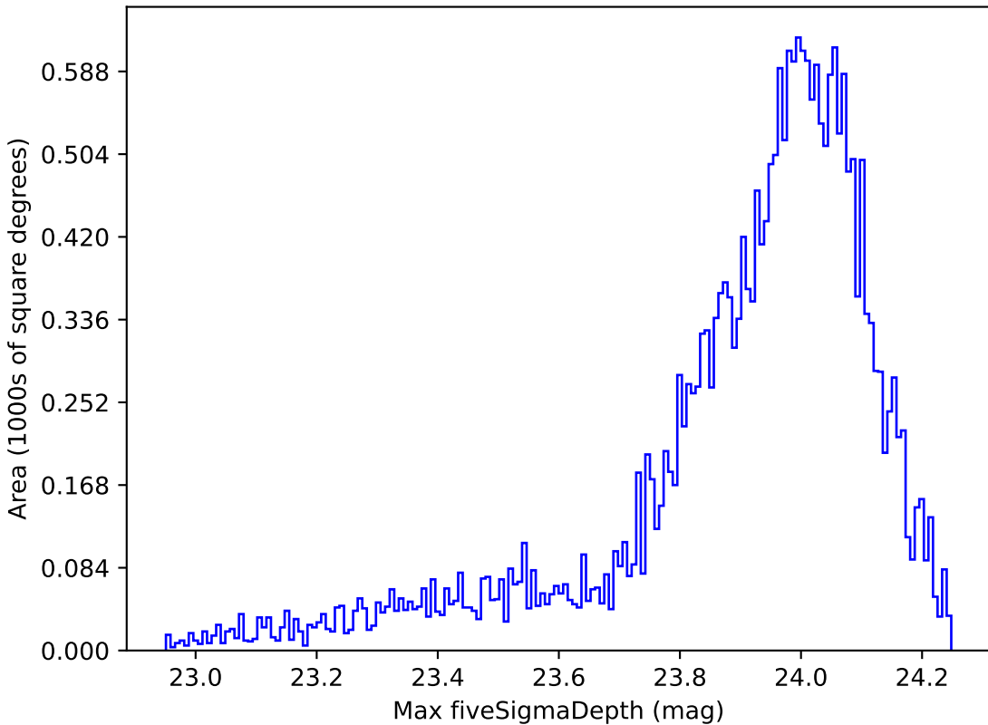
baseline_v2.1_10yrs Yr 1 i band: Max fiveSigmaDepth
