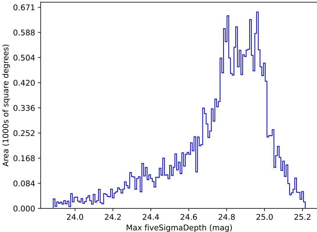
baseline_v2.1_10yrs Yr 1 g band: Max fiveSigmaDepth
