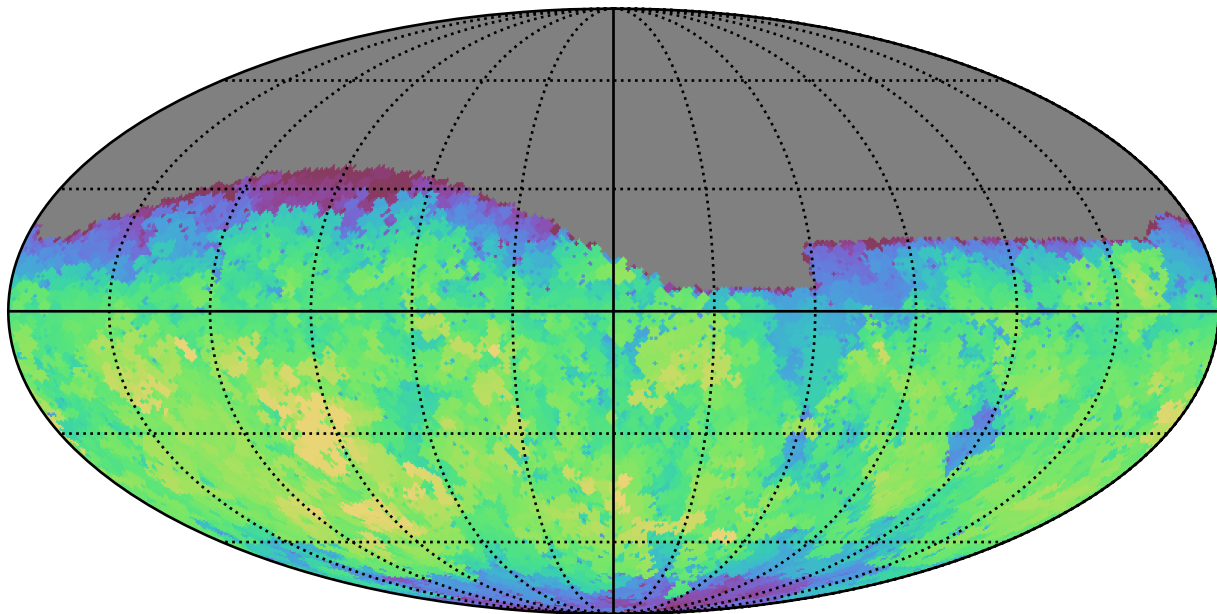
baseline_v2.1_10yrs Yr 1 all bands: Max fiveSigmaDepth
