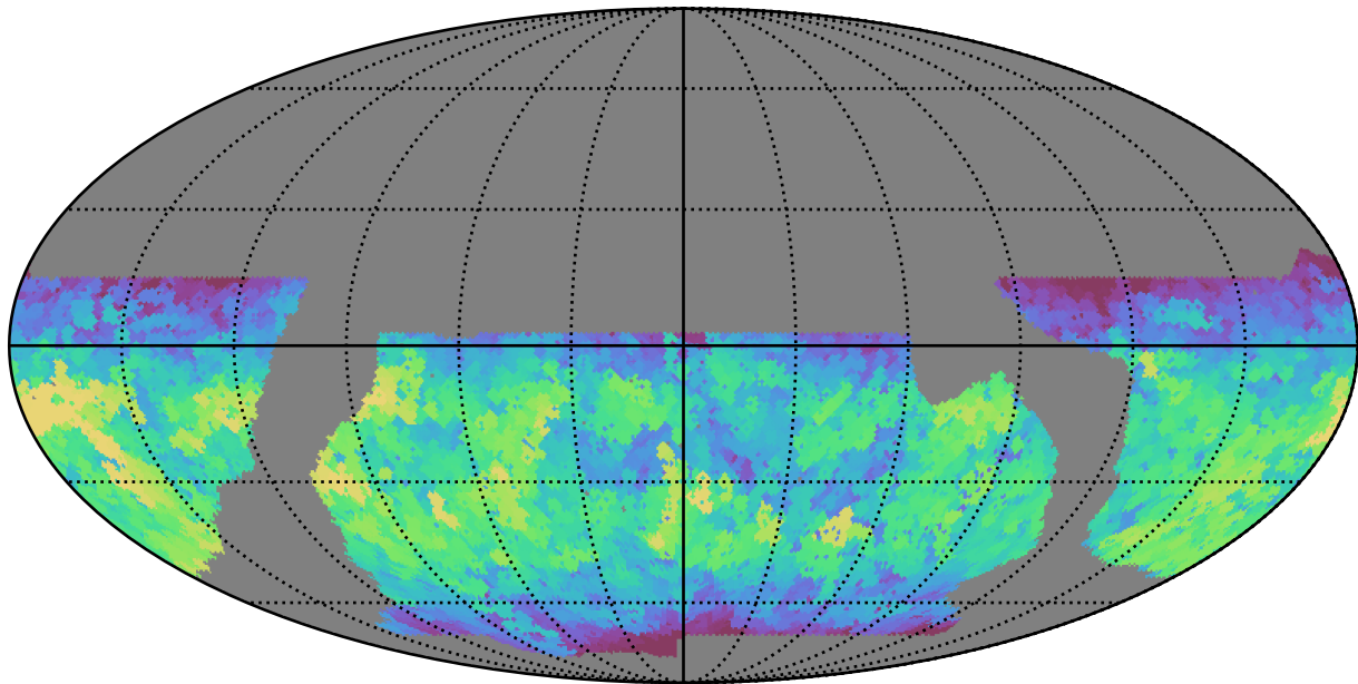
baseline_v2.1_10yrs WFD z band: Max fiveSigmaDepth
