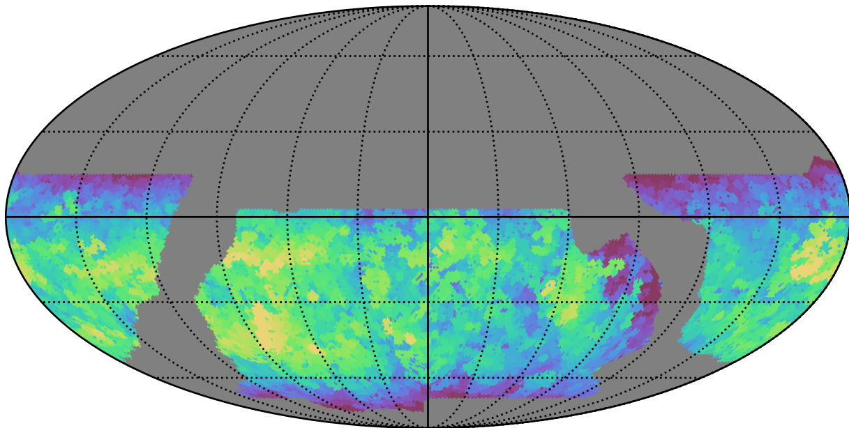
baseline_v2.1_10yrs WFD y band: Max fiveSigmaDepth
