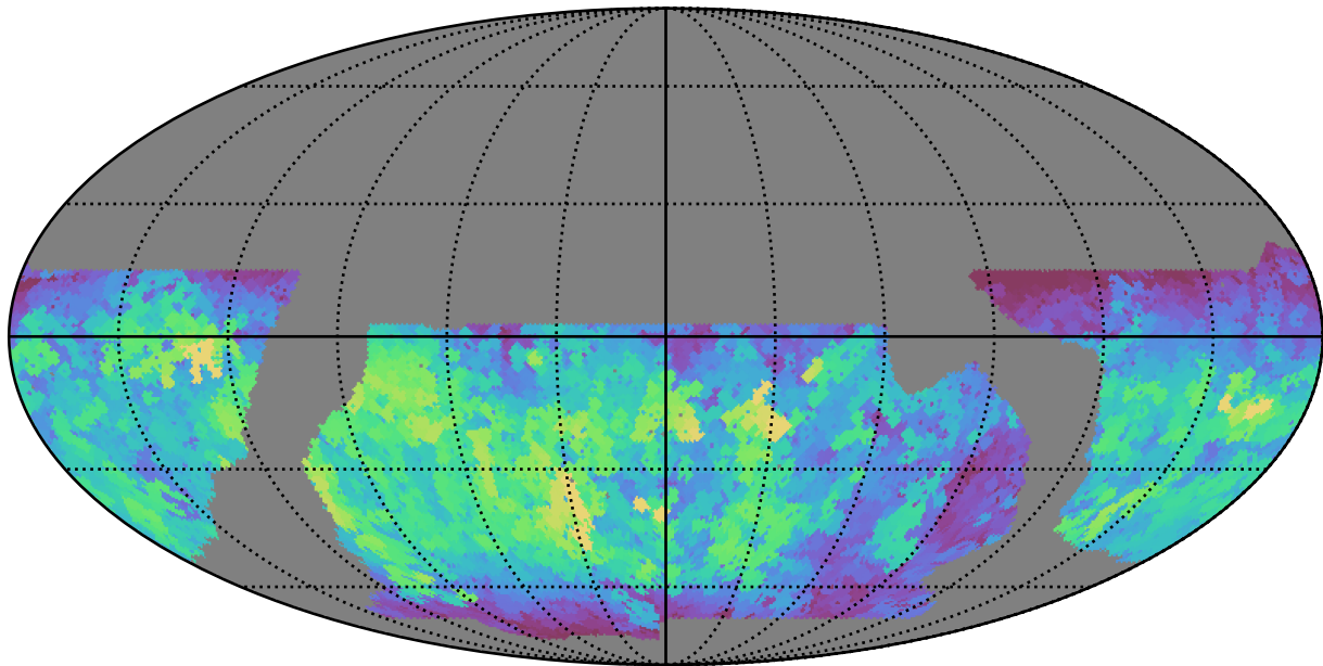
baseline_v2.1_10yrs WFD u band: Max fiveSigmaDepth
