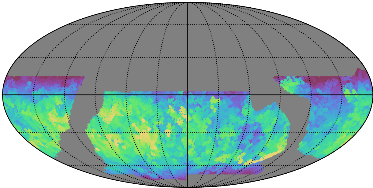
baseline_v2.1_10yrs WFD r band: Max fiveSigmaDepth
