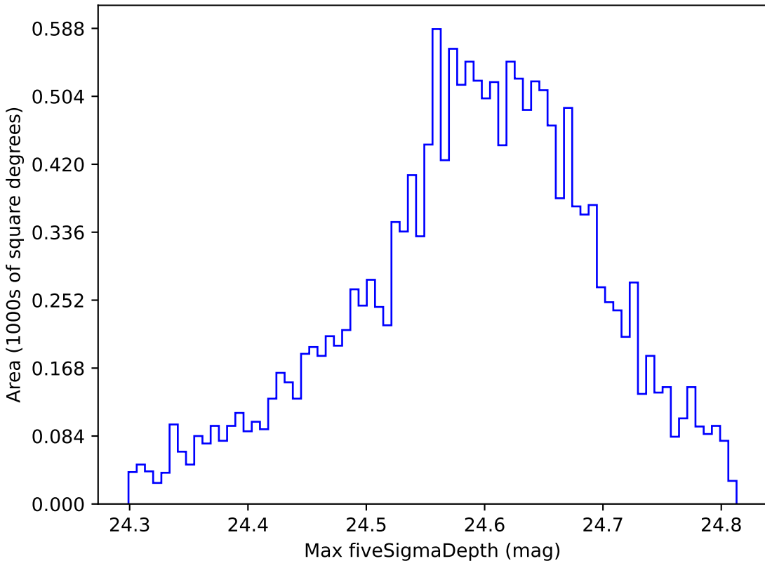
baseline_v2.1_10yrs WFD r band: Max fiveSigmaDepth
