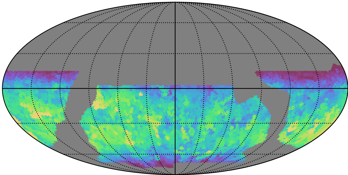
baseline_v2.1_10yrs WFD i band: Max fiveSigmaDepth
