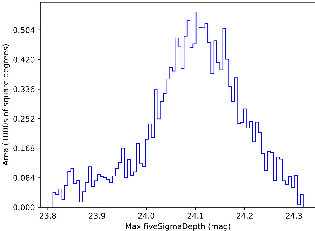
baseline_v2.1_10yrs WFD i band: Max fiveSigmaDepth
