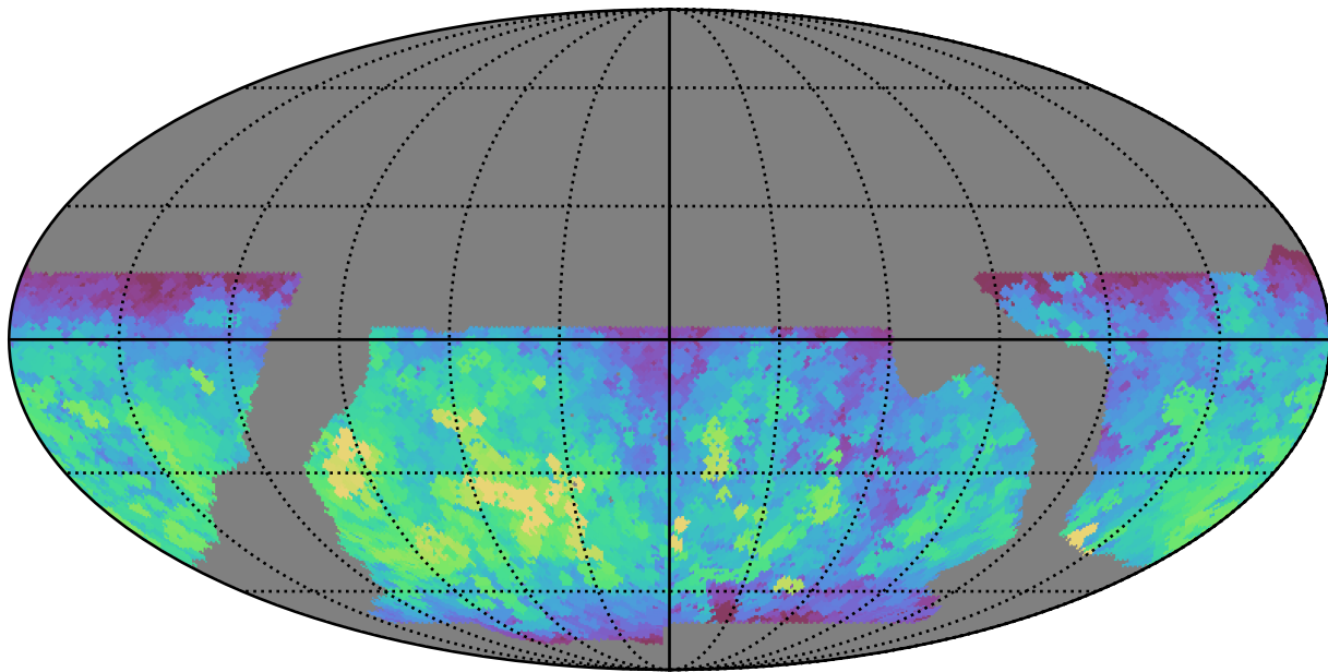
baseline_v2.1_10yrs WFD g band: Max fiveSigmaDepth
