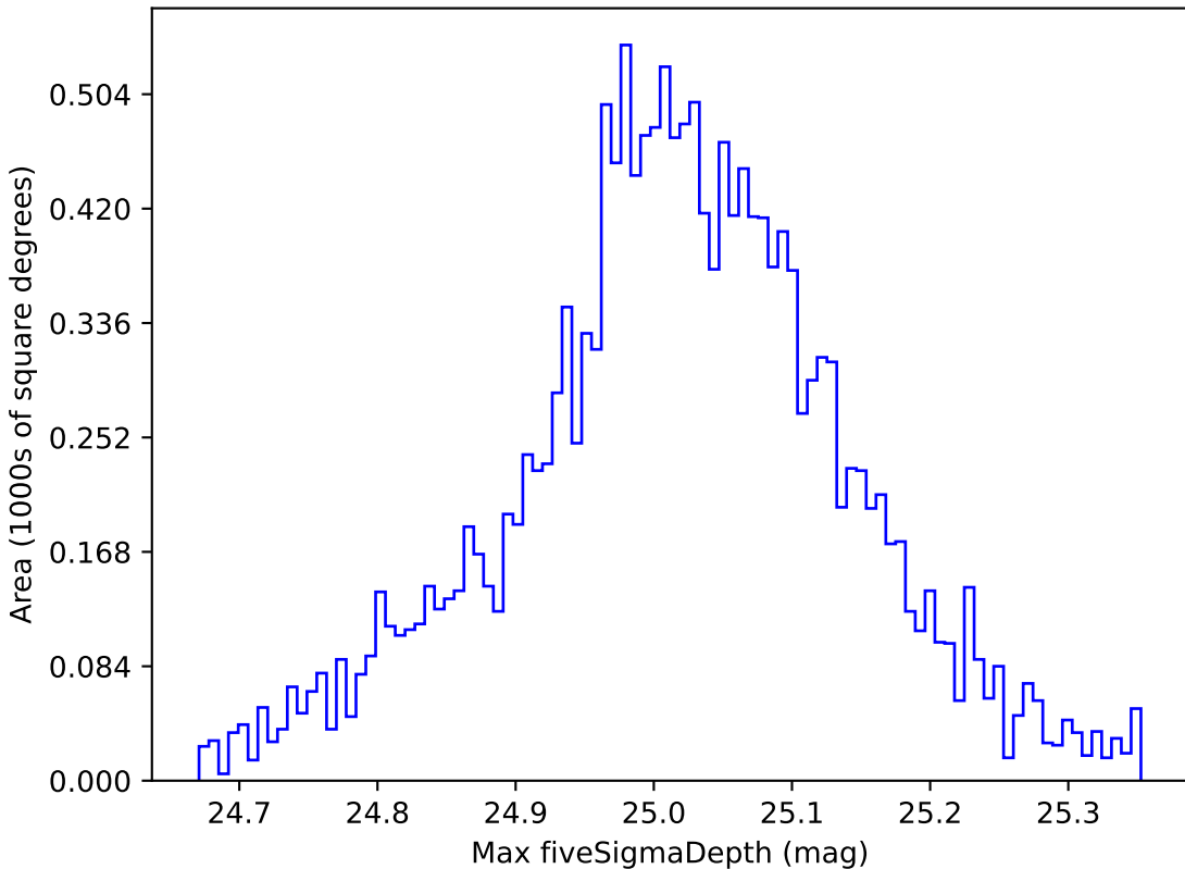
baseline_v2.1_10yrs WFD g band: Max fiveSigmaDepth
