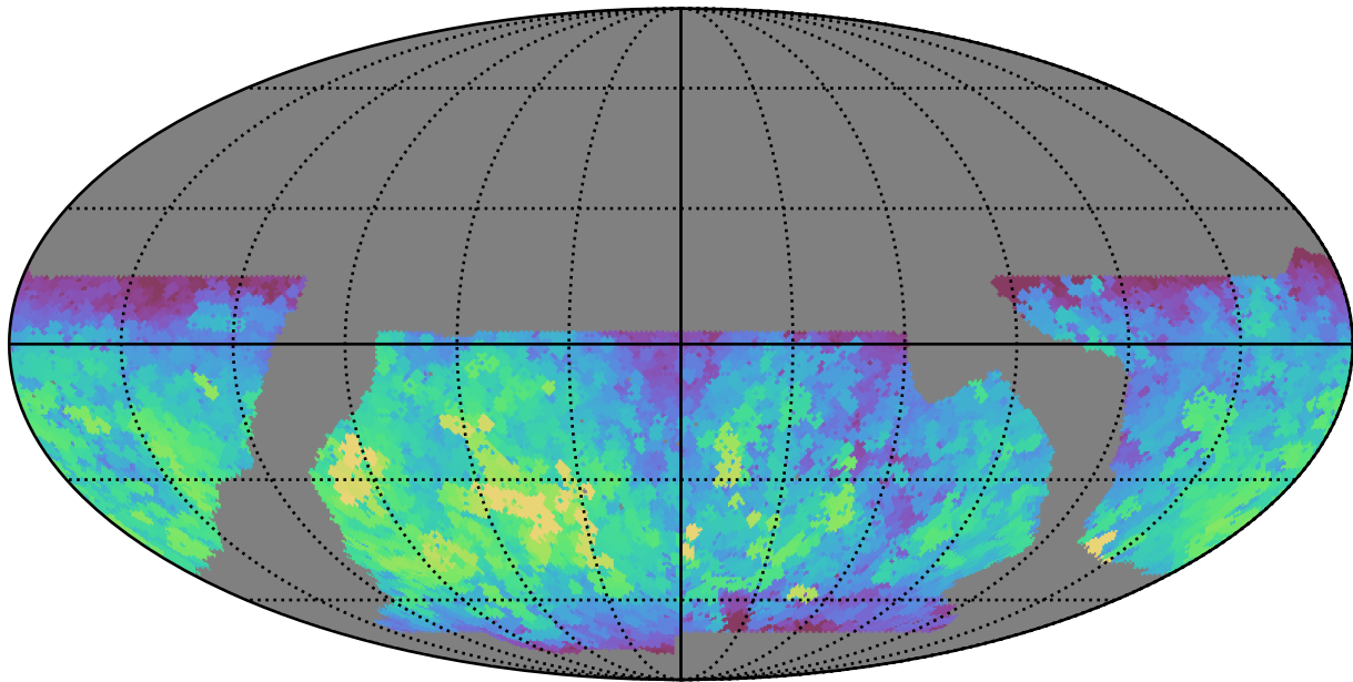
baseline_v2.1_10yrs WFD all bands: Max fiveSigmaDepth
