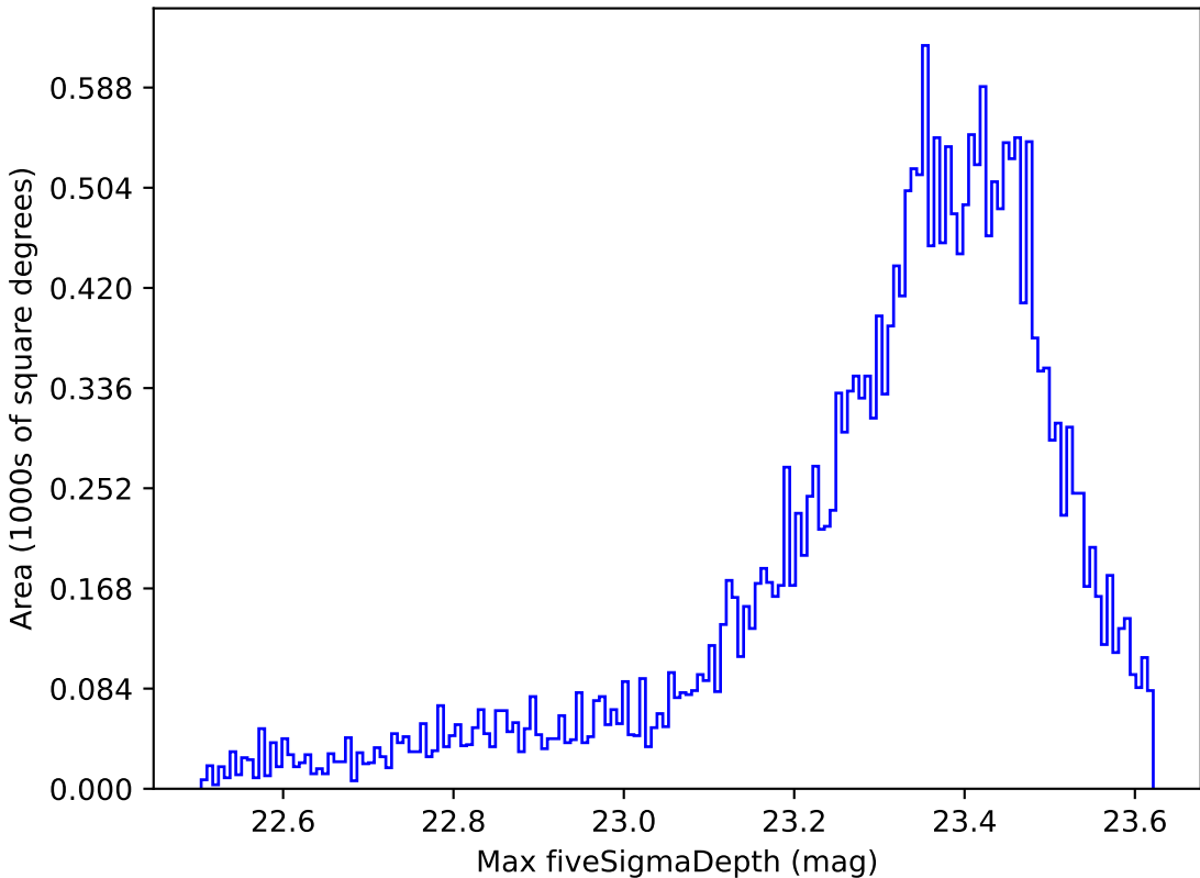
baseline_v2.1_10yrs All sky z band: Max fiveSigmaDepth
