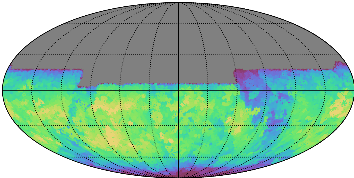
baseline_v2.1_10yrs All sky y band: Max fiveSigmaDepth
