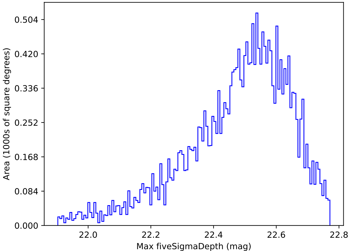
baseline_v2.1_10yrs All sky y band: Max fiveSigmaDepth
