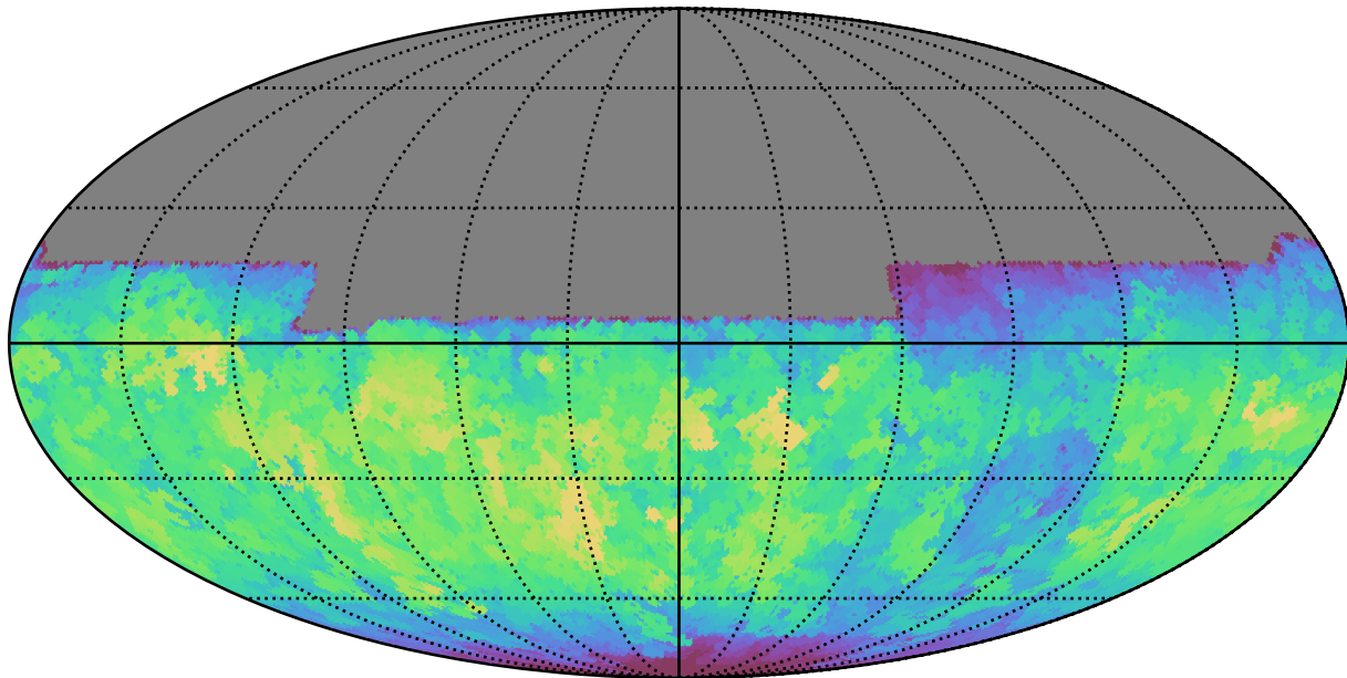
baseline_v2.1_10yrs All sky u band: Max fiveSigmaDepth
