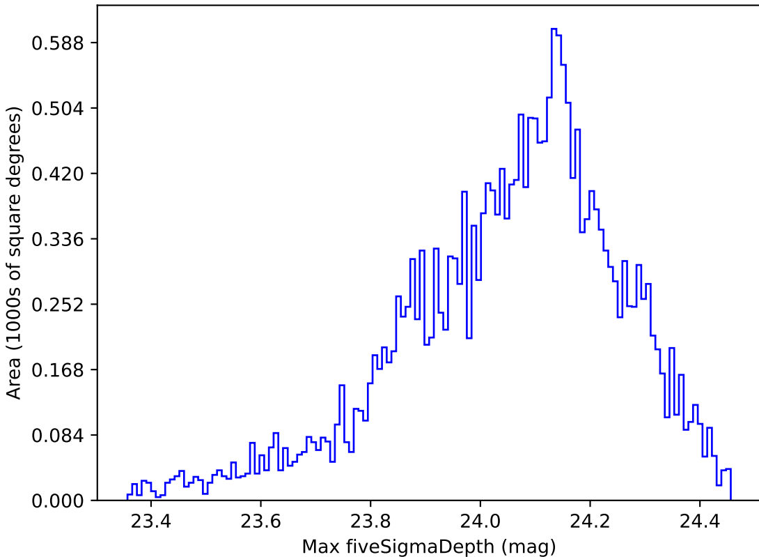
baseline_v2.1_10yrs All sky u band: Max fiveSigmaDepth
