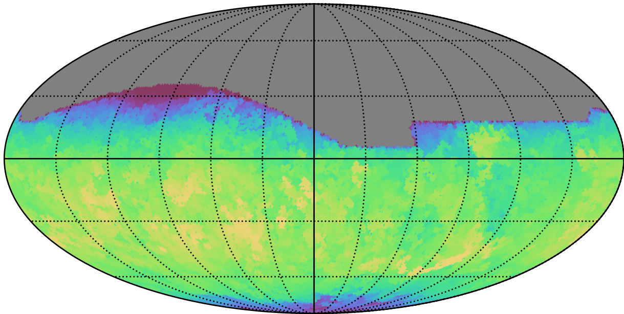
baseline_v2.1_10yrs All sky r band: Max fiveSigmaDepth
