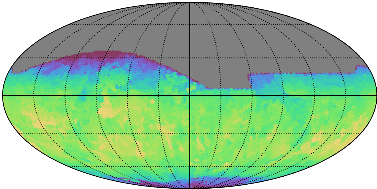
baseline_v2.1_10yrs All sky i band: Max fiveSigmaDepth
