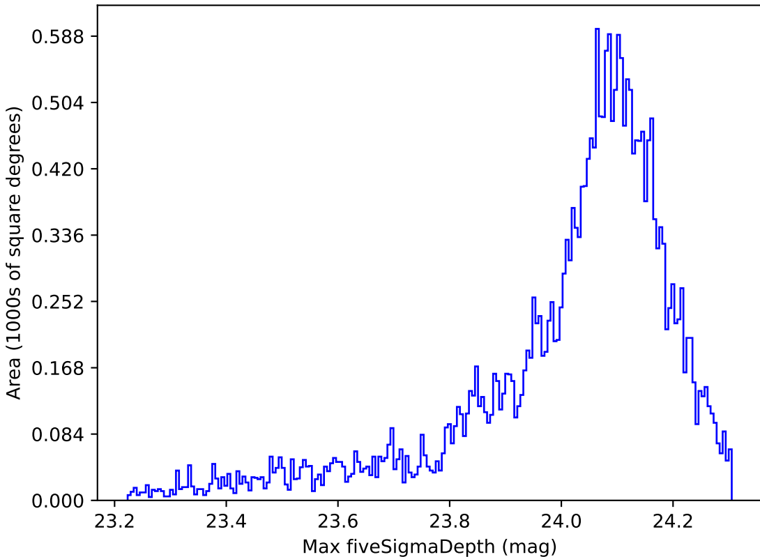
baseline_v2.1_10yrs All sky i band: Max fiveSigmaDepth
