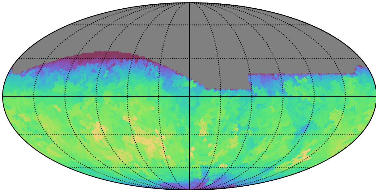
baseline_v2.1_10yrs All sky g band: Max fiveSigmaDepth
