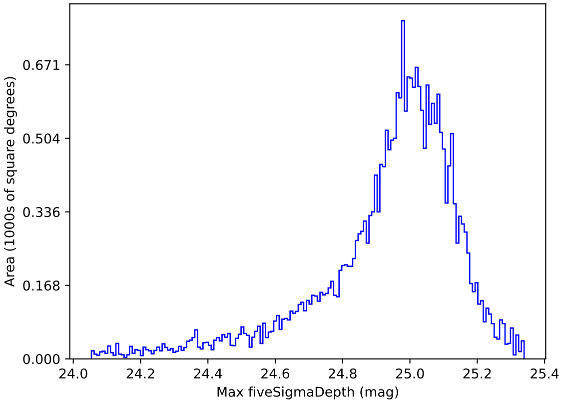
baseline_v2.1_10yrs All sky g band: Max fiveSigmaDepth
