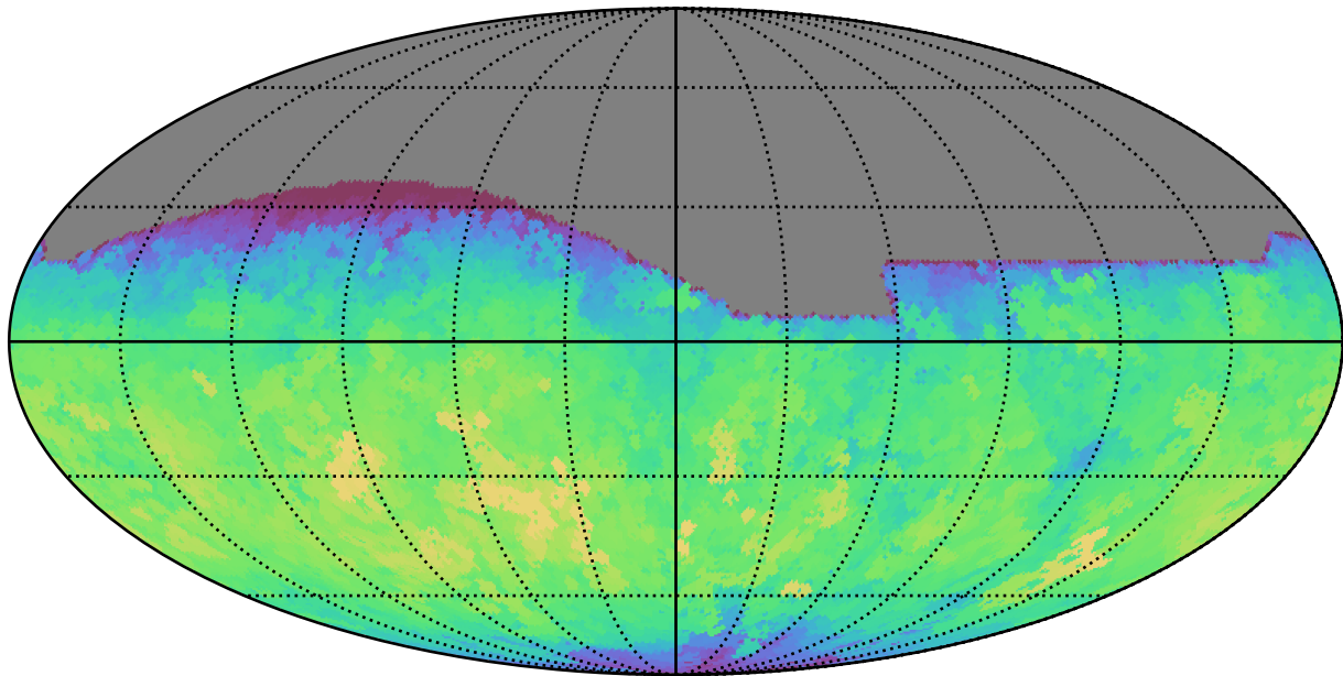
baseline_v2.1_10yrs All sky all bands: Max fiveSigmaDepth
