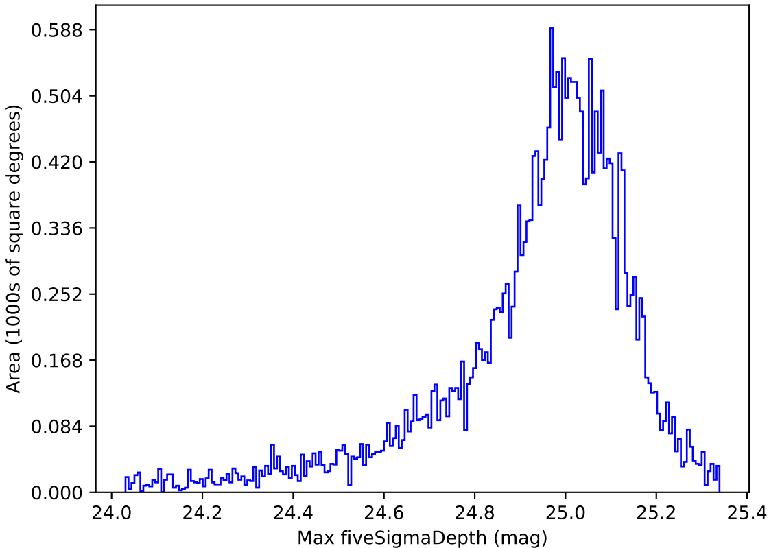
baseline_v2.1_10yrs All sky all bands: Max fiveSigmaDepth
