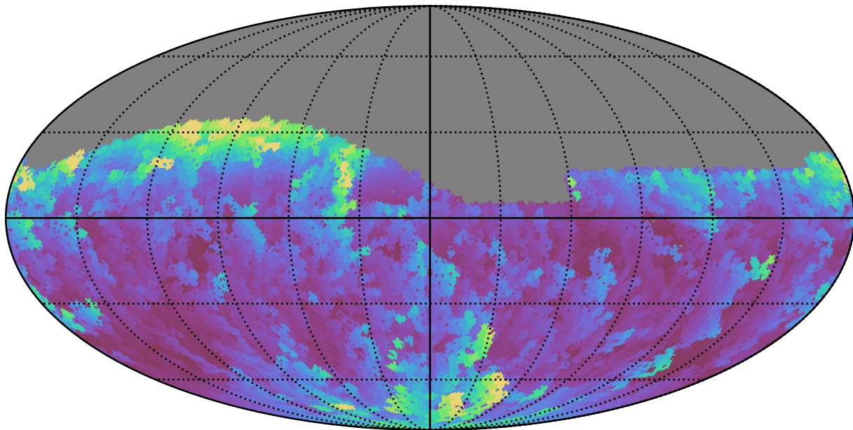
baseline_v2.1_10yrs Yr 1 z band: Max airmass
