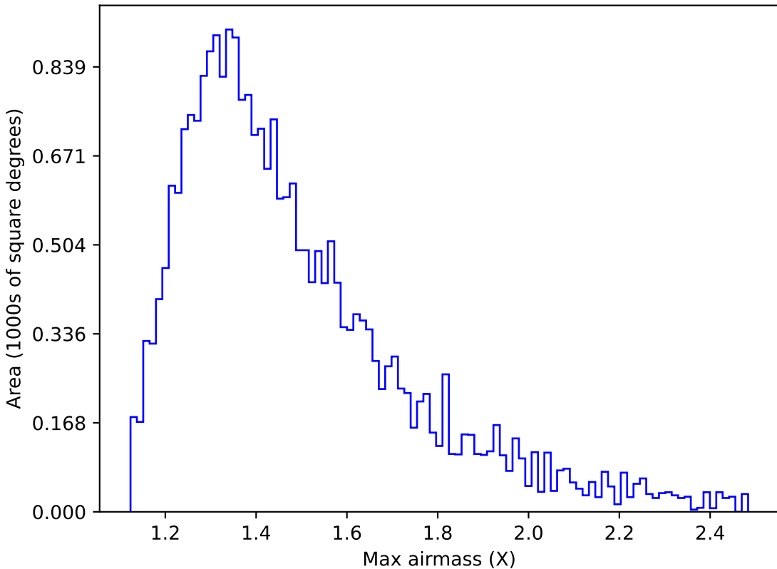
baseline_v2.1_10yrs Yr 1 z band: Max airmass
