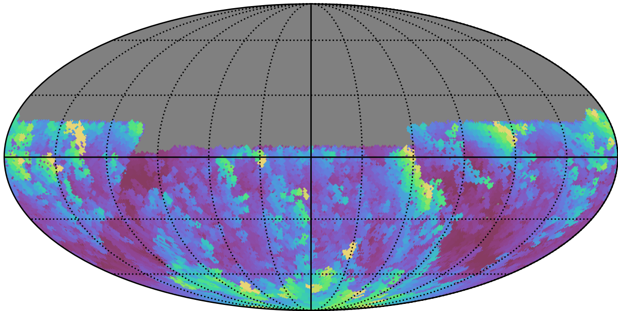
baseline_v2.1_10yrs Yr 1 y band: Max airmass
