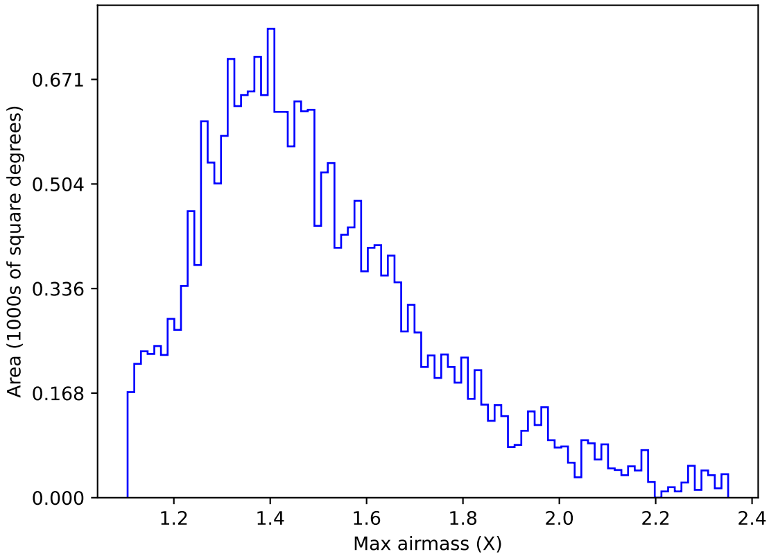
baseline_v2.1_10yrs Yr 1 y band: Max airmass
