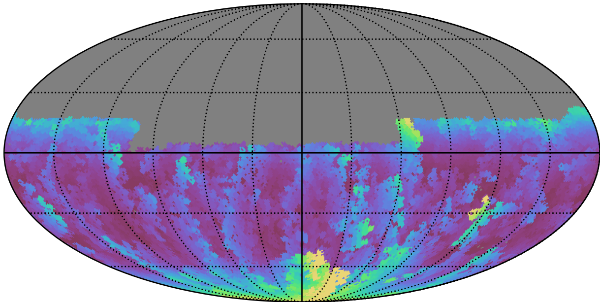
baseline_v2.1_10yrs Yr 1 u band: Max airmass
