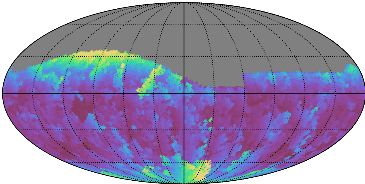
baseline_v2.1_10yrs Yr 1 r band: Max airmass
