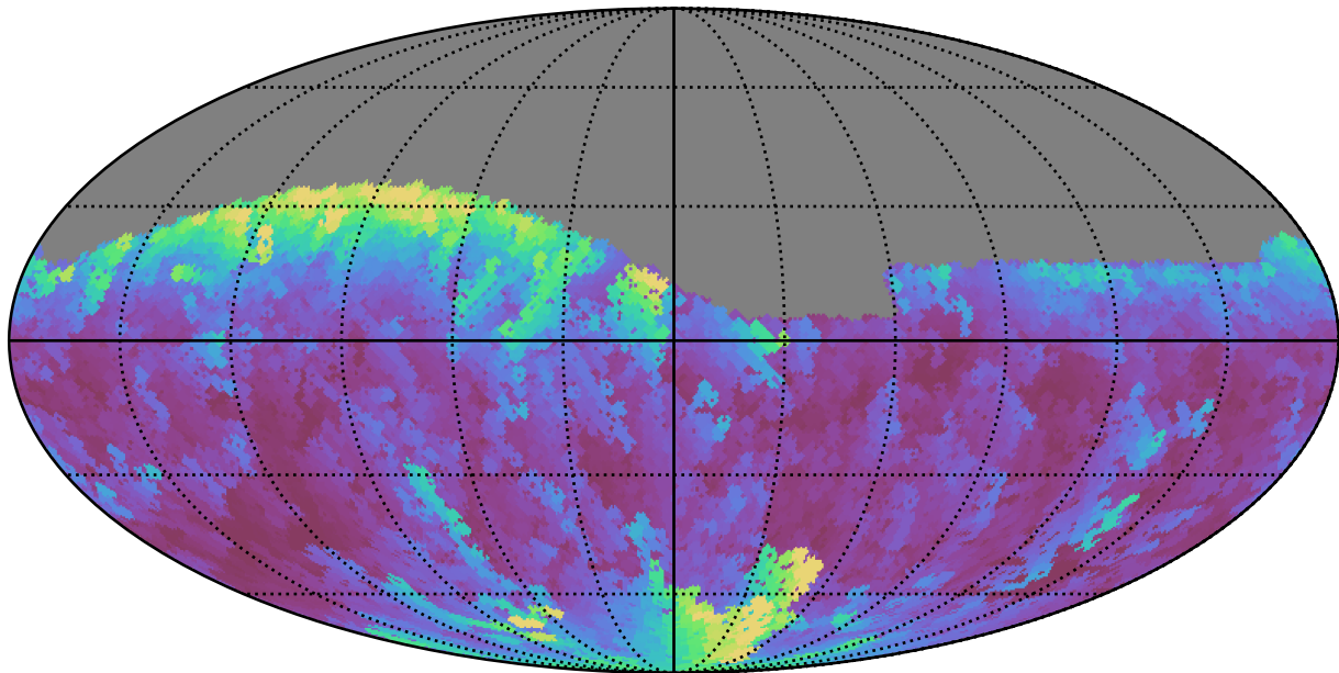
baseline_v2.1_10yrs Yr 1 i band: Max airmass
