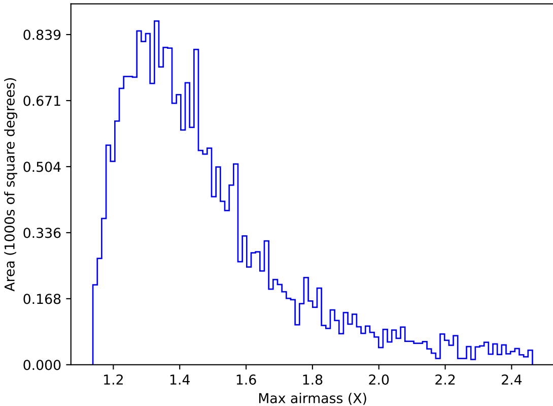
baseline_v2.1_10yrs Yr 1 i band: Max airmass
