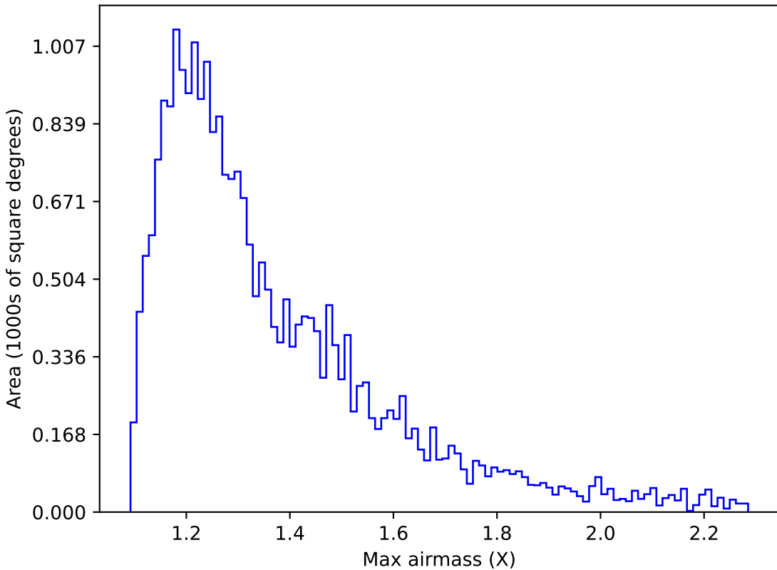
baseline_v2.1_10yrs Yr 1 g band: Max airmass
