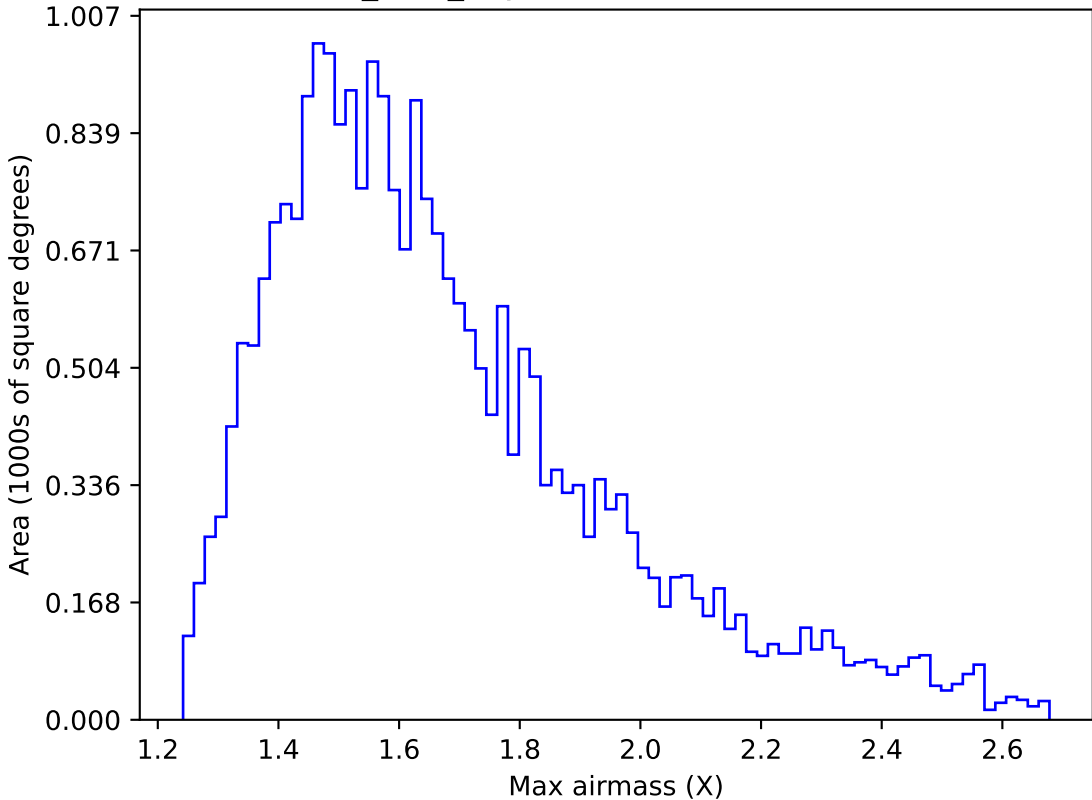
baseline_v2.1_10yrs Yr 1 all bands: Max airmass
