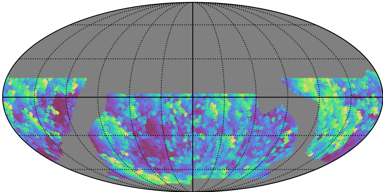
baseline_v2.1_10yrs WFD z band: Max airmass
