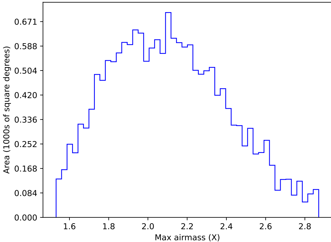
baseline_v2.1_10yrs WFD z band: Max airmass
