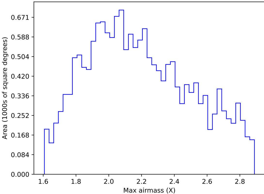
baseline_v2.1_10yrs WFD y band: Max airmass
