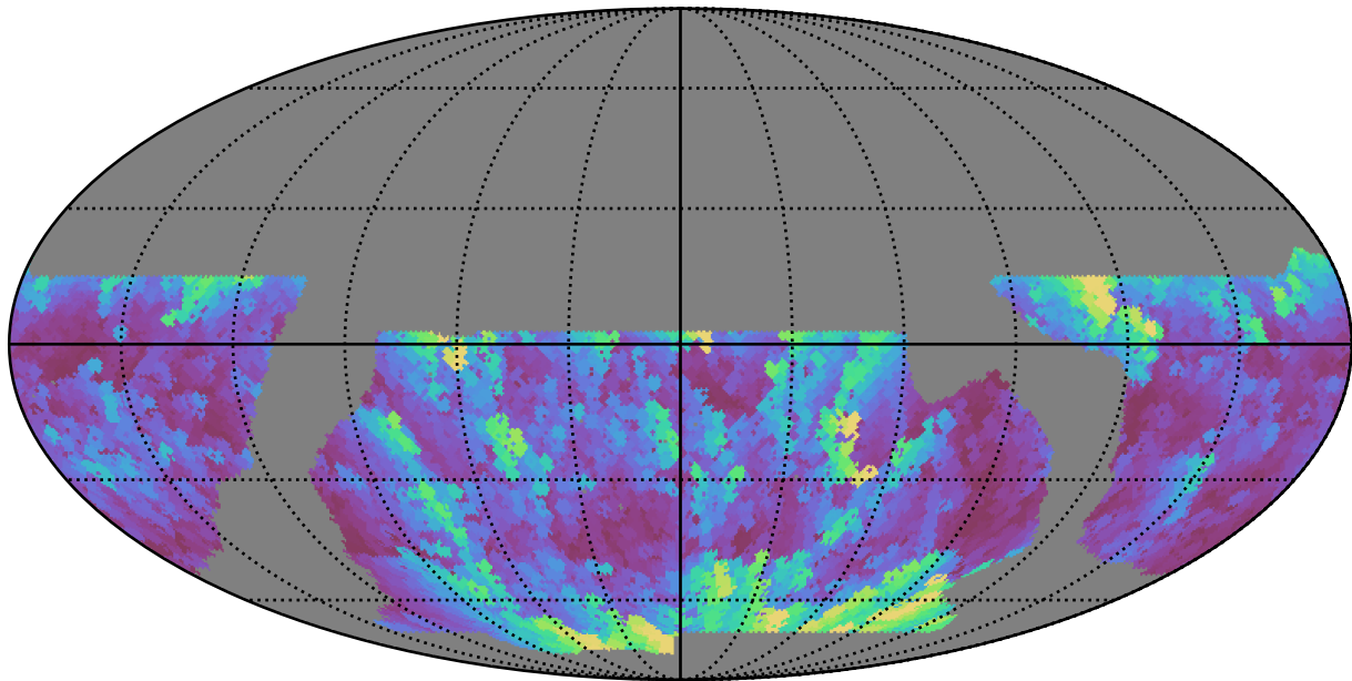
baseline_v2.1_10yrs WFD u band: Max airmass
