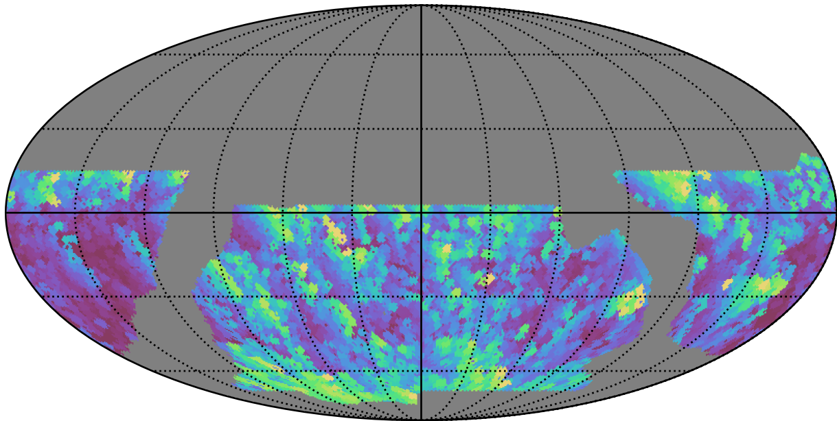
baseline_v2.1_10yrs WFD r band: Max airmass
