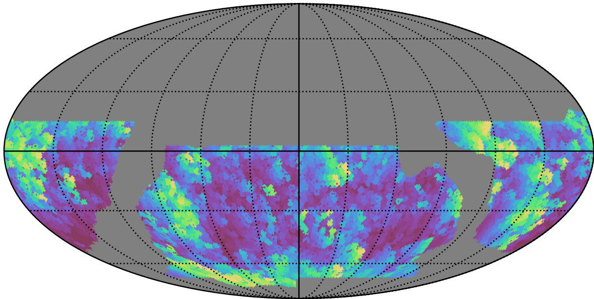
baseline_v2.1_10yrs WFD i band: Max airmass
