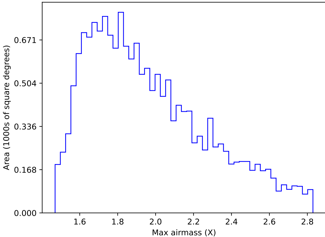
baseline_v2.1_10yrs WFD i band: Max airmass
