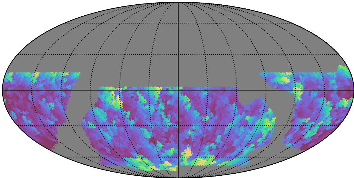
baseline_v2.1_10yrs WFD g band: Max airmass
